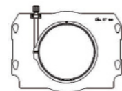
Clamp Adapter K2.47241.0 (ø 95 mm)
